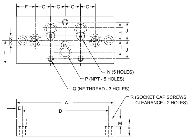
BOTTOM PORTED
